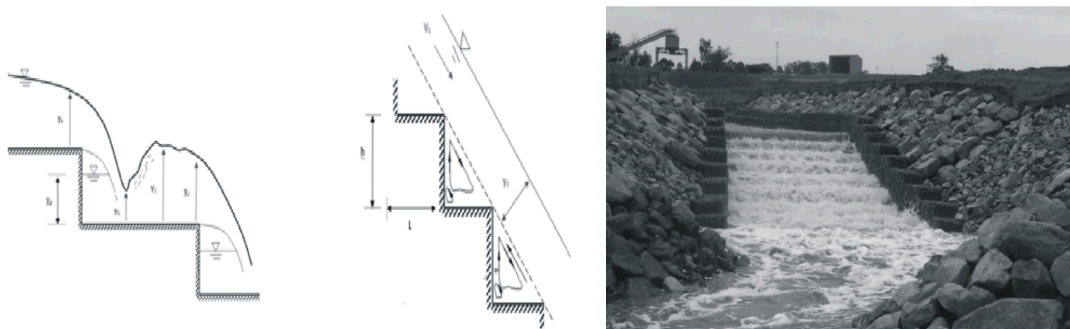
Fig. 1: Type of flow on step spillway
