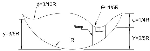
FIG. 2: Approximate dimensions of the Duguay-Hannaford baffle relative to the culvert radius, R .
