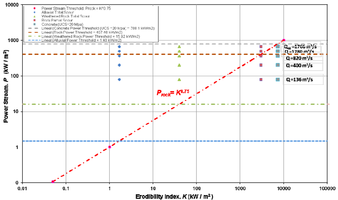
Figure 8: Half-height outlet. Stream power of the jet for different flows as a function of the erodibility: alluvial, weathered rock, intact rock and concrete cases (Water cushion depth 24 m)
