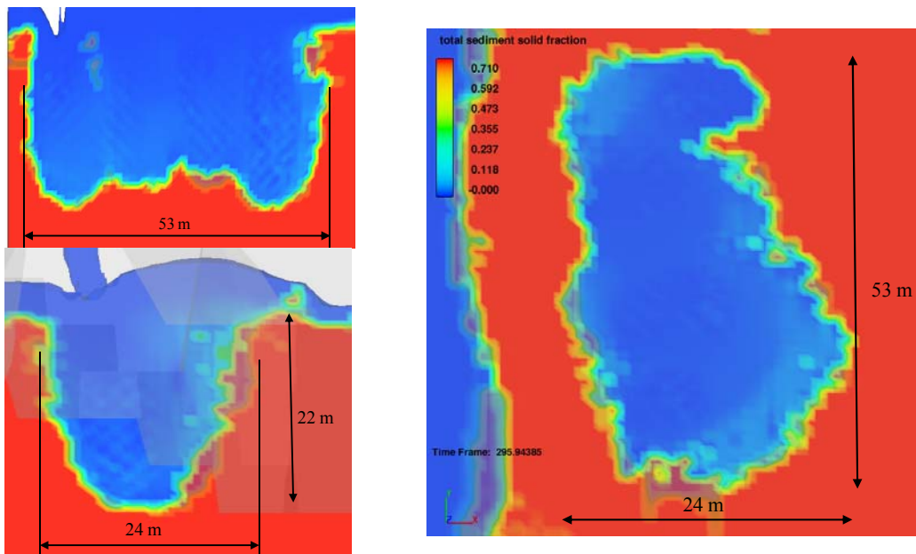
Figure 10: Front, lateral, and top view of the scour due to the free surface weir
